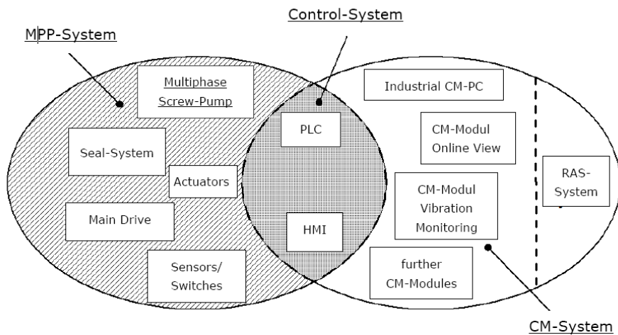
figure 2: Control System of a MPP-Unit and additional CM-Hardware
